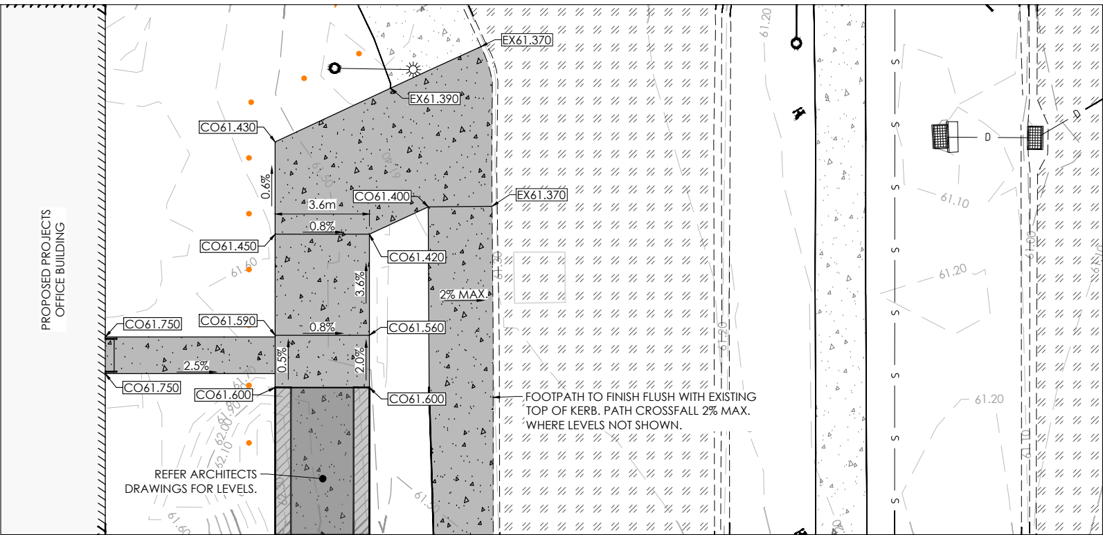
EASTERN PATHWAY LEVELS
