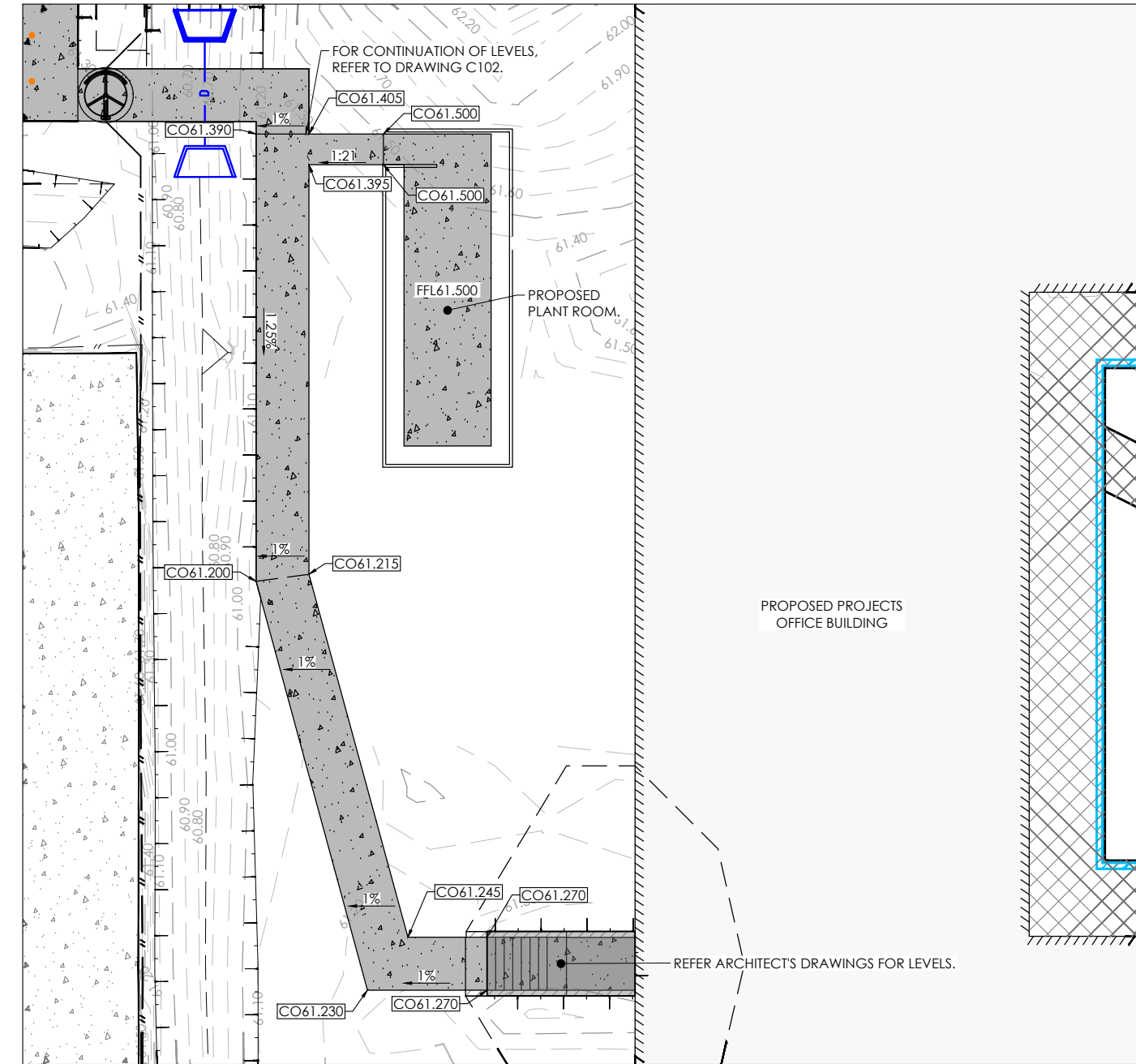
WESTERN PATHWAY LEVELS
